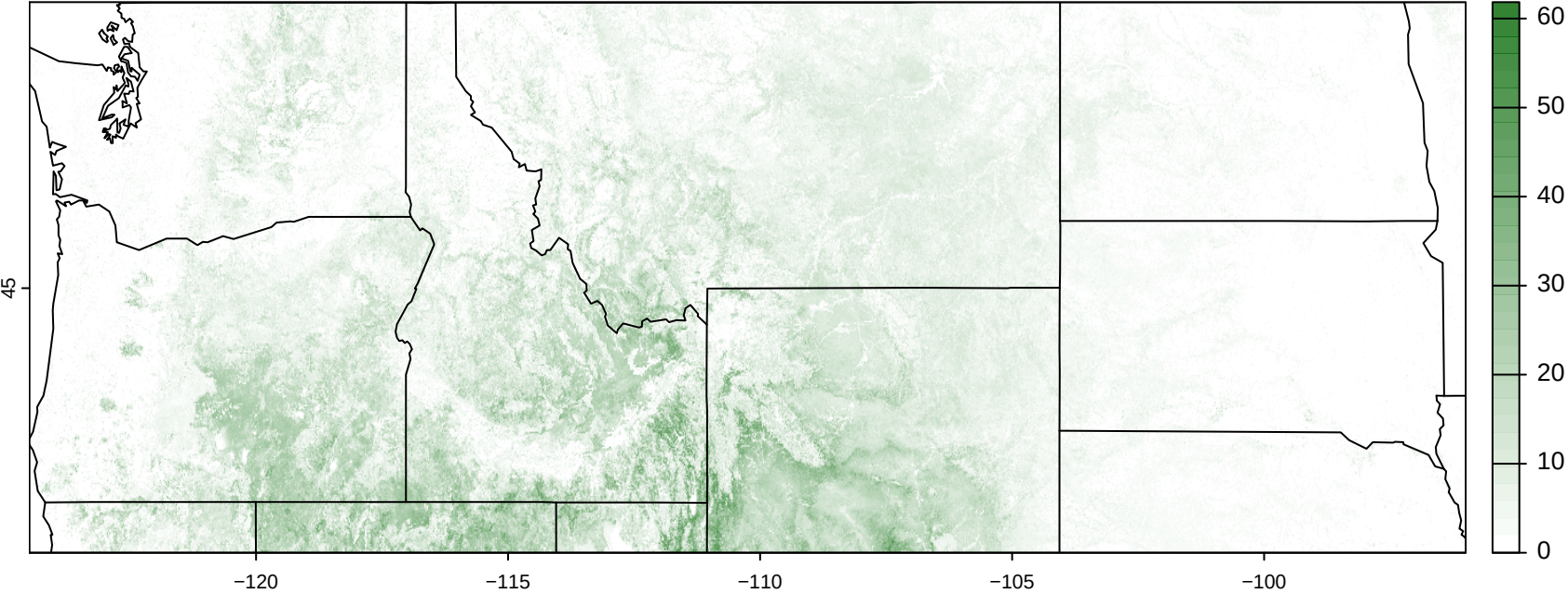
shrub cover % (2022)
