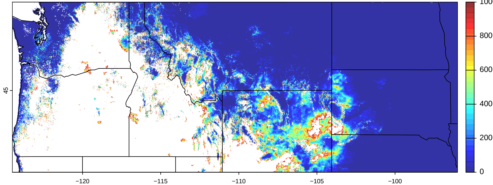
20240706 predicted acres potential new growth
