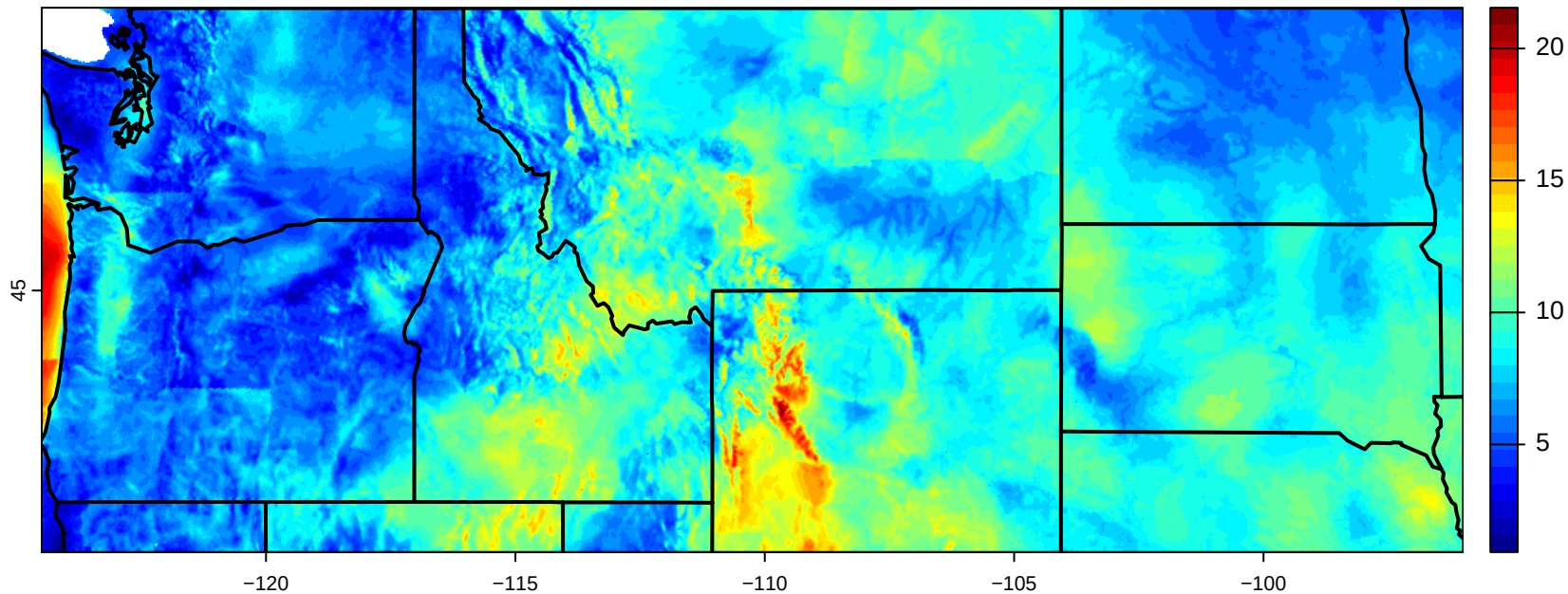
20240705 Avg wind speed 1200–1800 hrs
