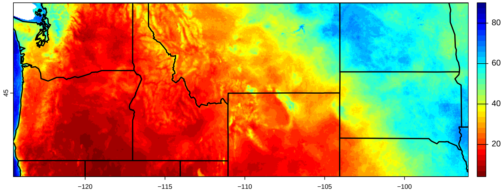
20240705 Minimum RH
