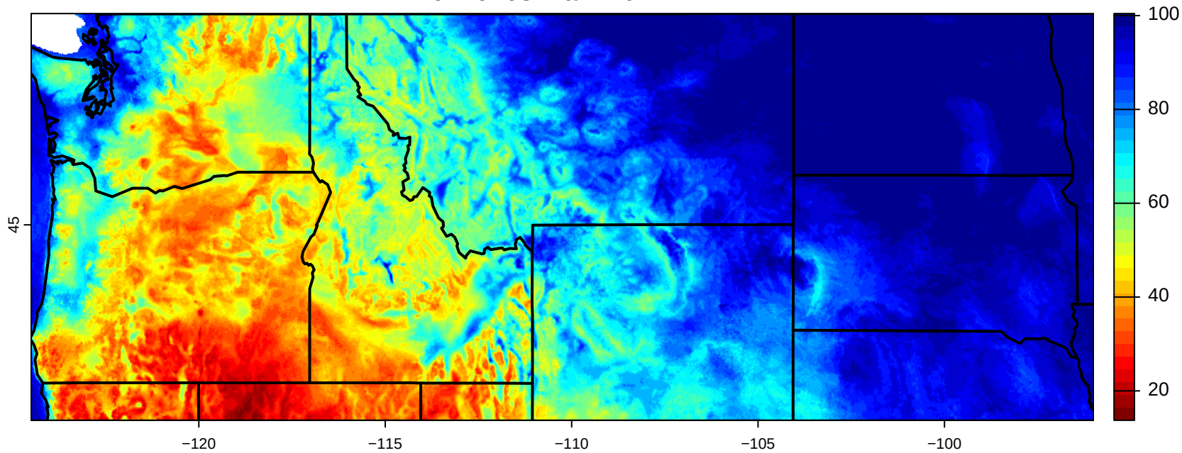
20240705 Maximum RH
