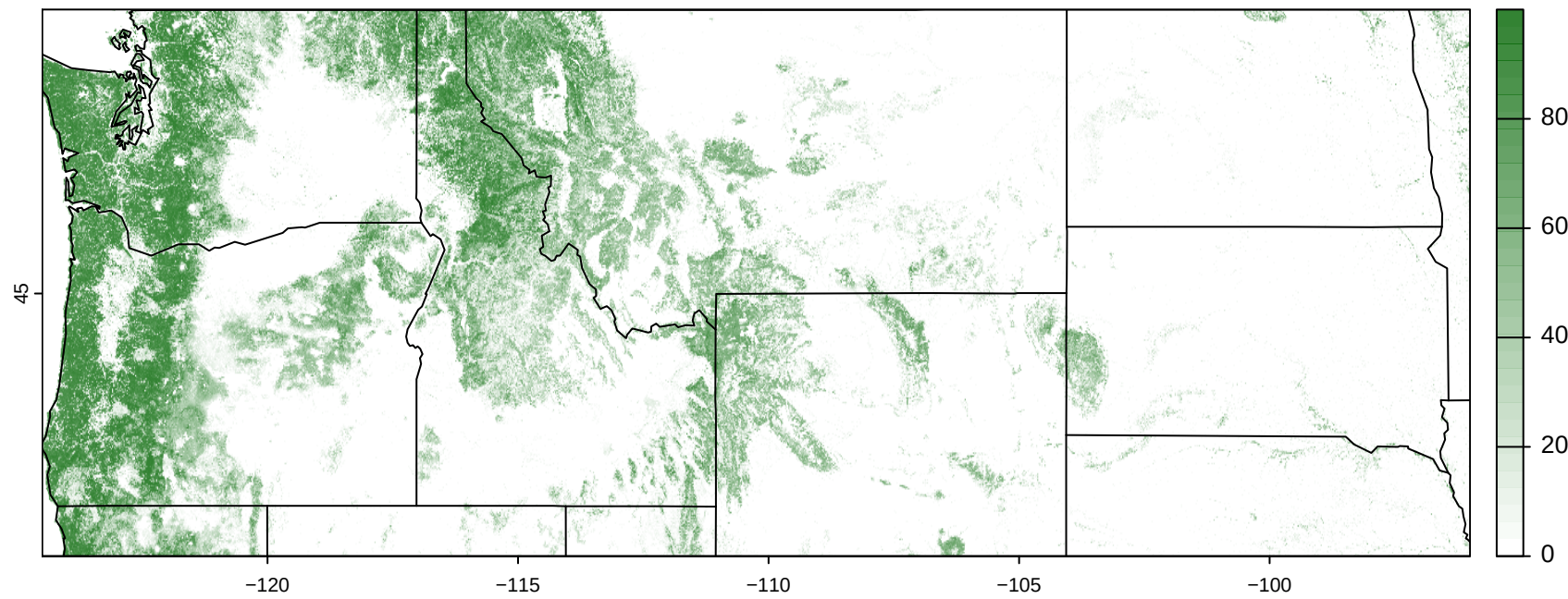
forest cover % (2022)
