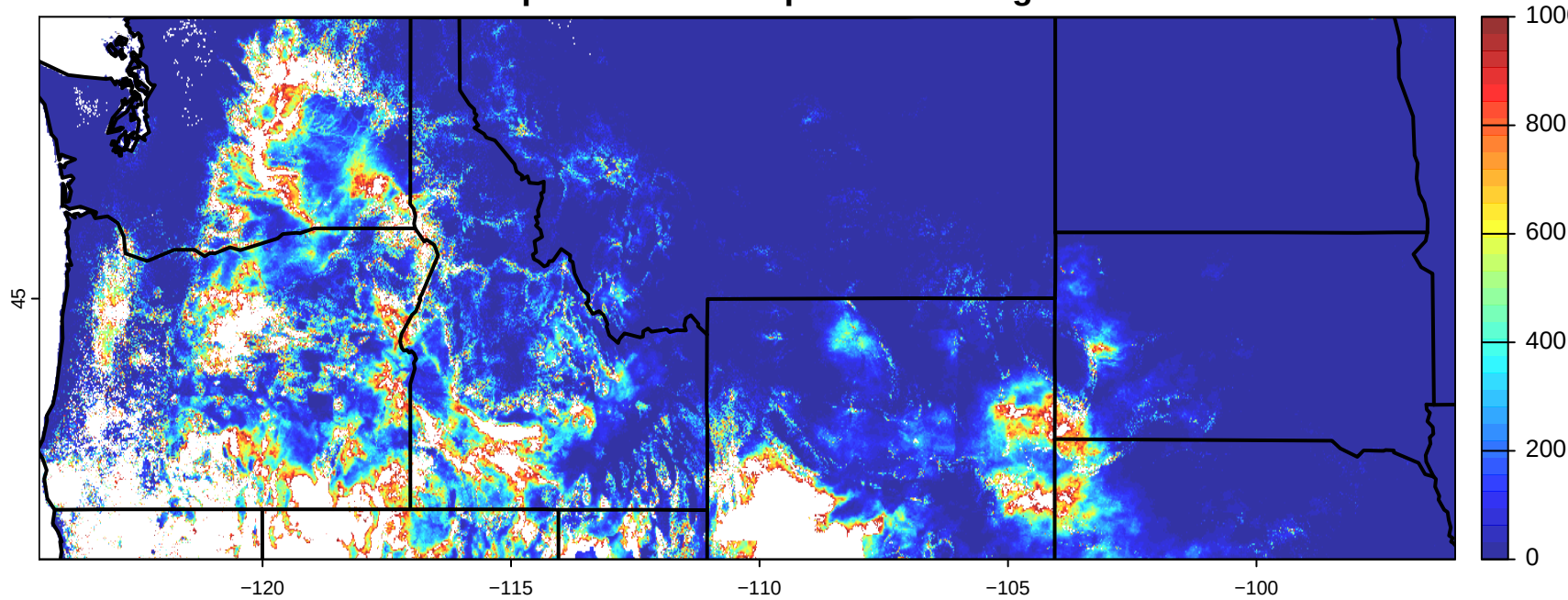
20240704 predicted acres potential new growth
