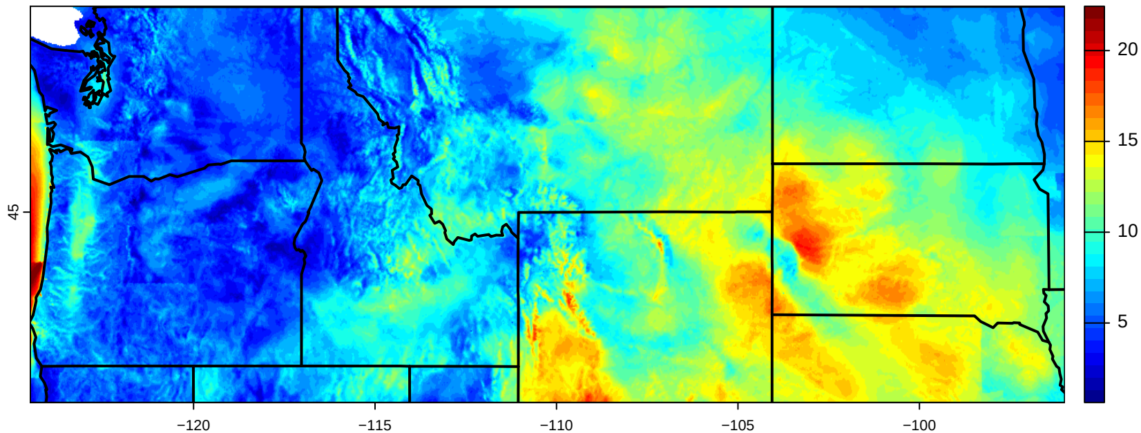
20240704 Avg wind speed 1200–1800 hrs
