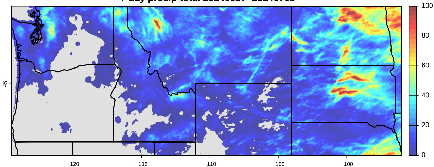
7 day precip total 20240627-20240703
