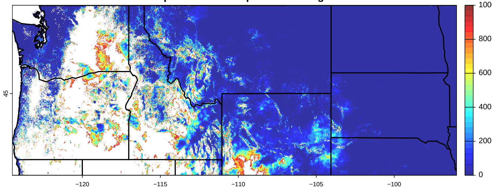
20240705 predicted acres potential new growth
