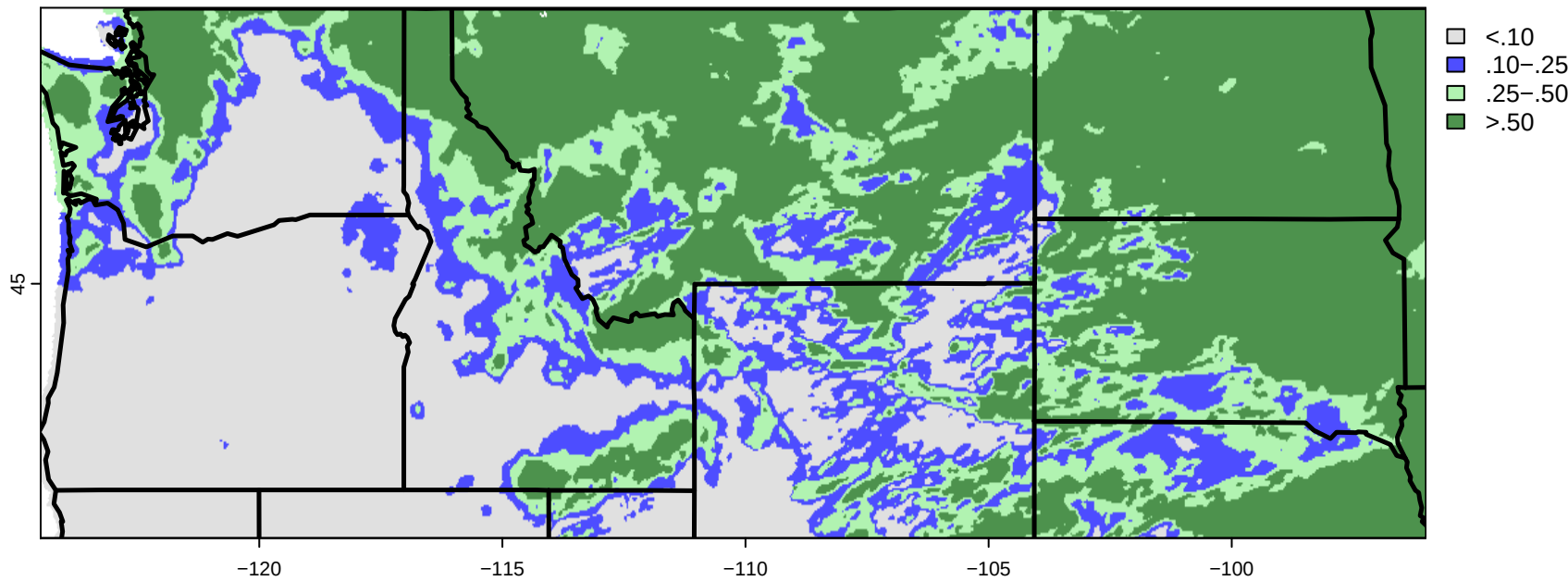
7 day precipitation total (inches)
