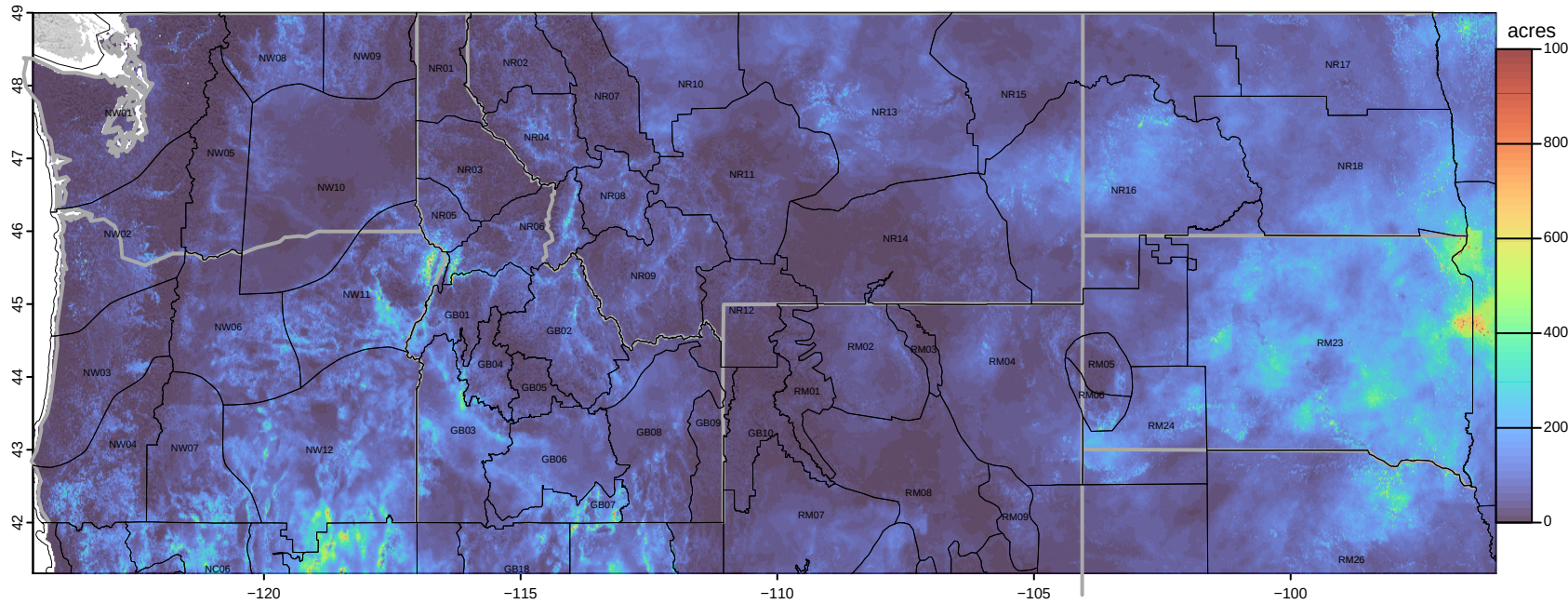
20250510 potential acres fire growth
