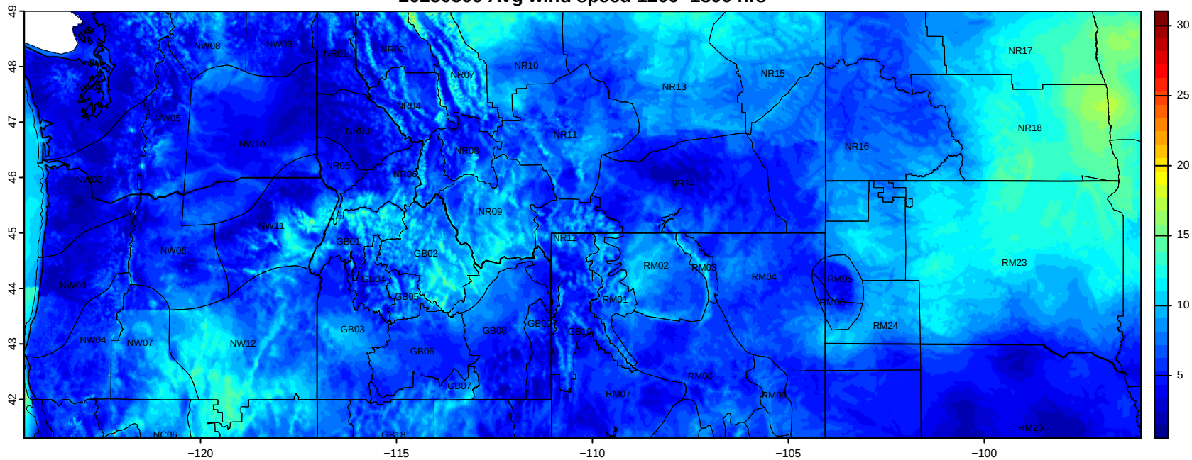
20250510 Avg wind speed 1200–1800 hrs
