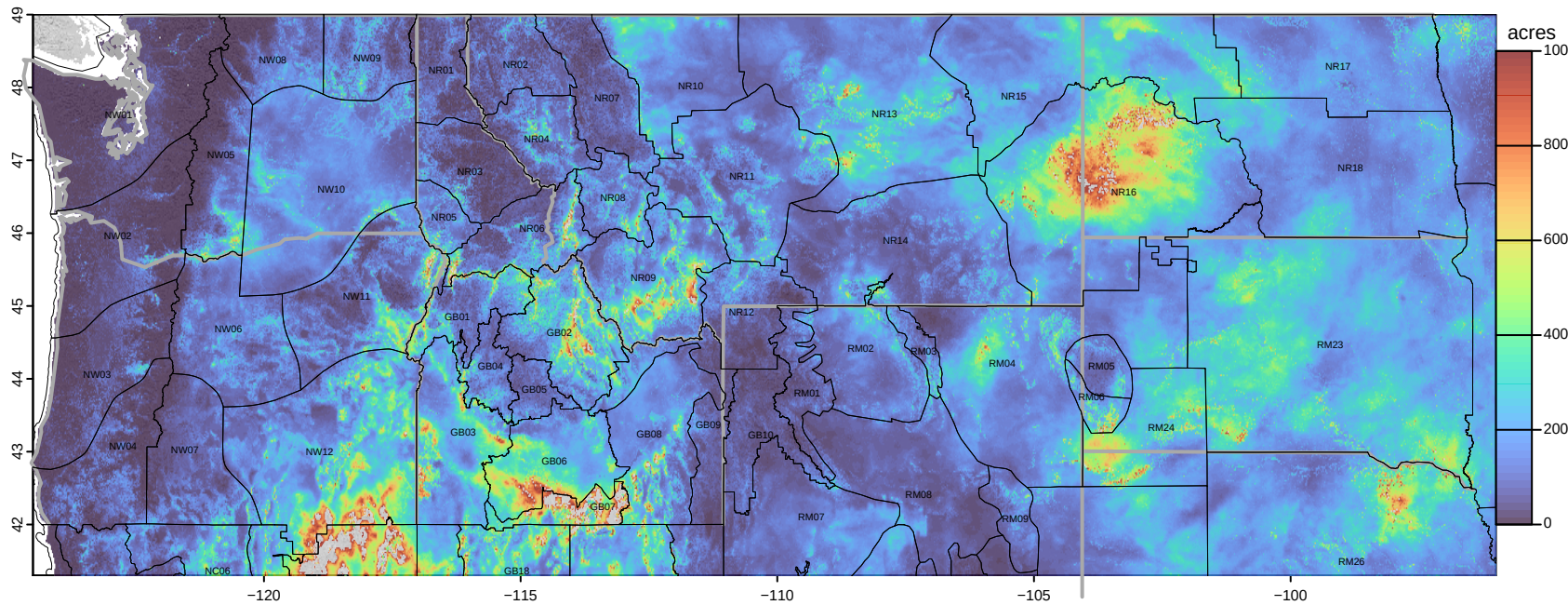
20250511 potential acres fire growth
