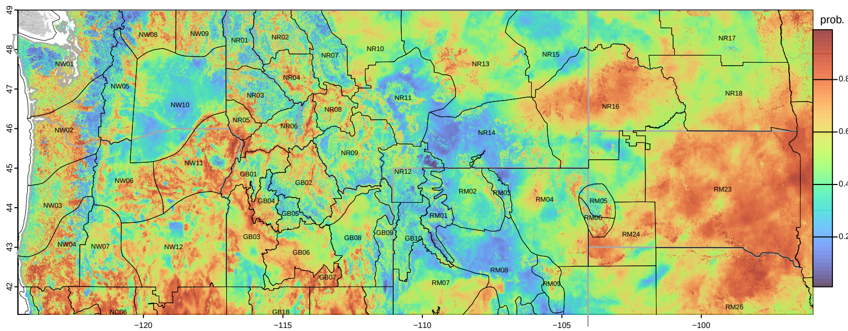
20250510 Probability. of fire spread > 70 acres
