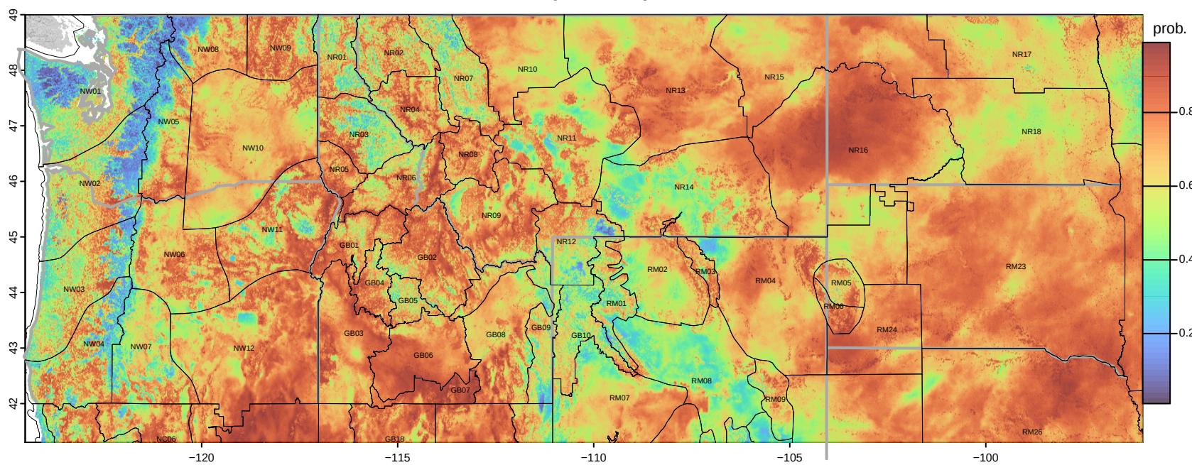
20250511 Probability. of fire spread > 70 acres
