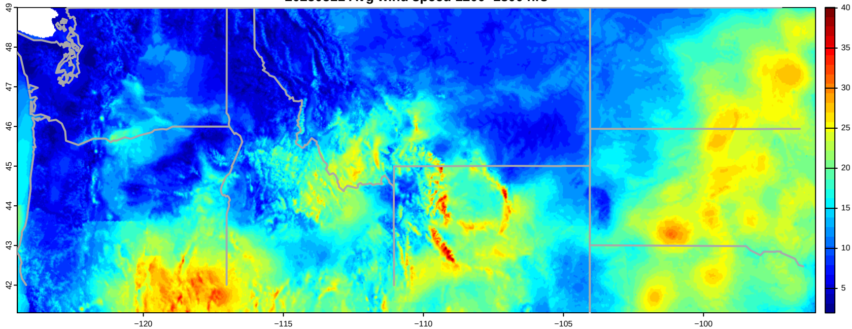
20250511 Avg wind speed 1200–1800 hrs
