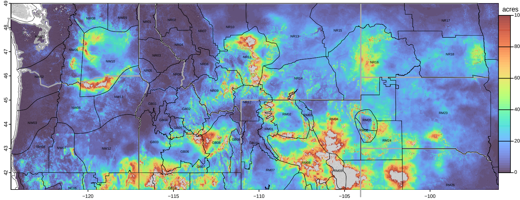
20260910 potential acres fire growth
