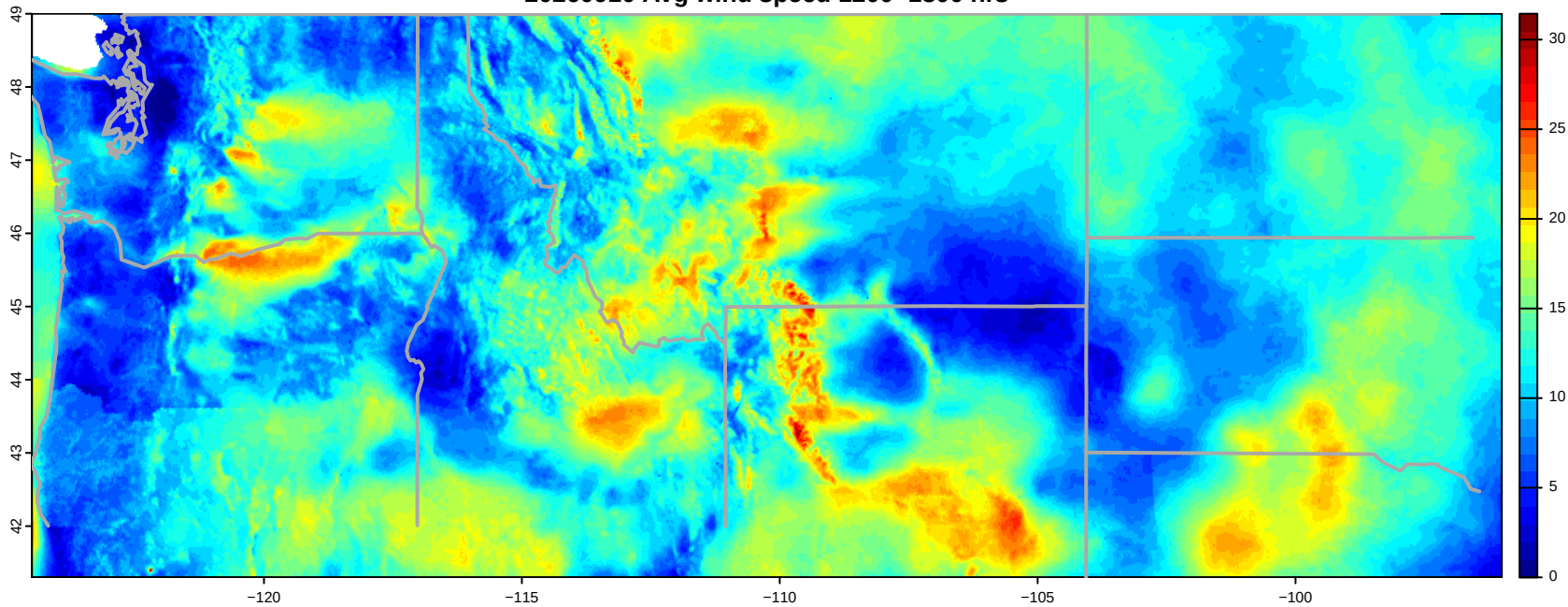
20260910 Avg wind speed 1200–1800 hrs
