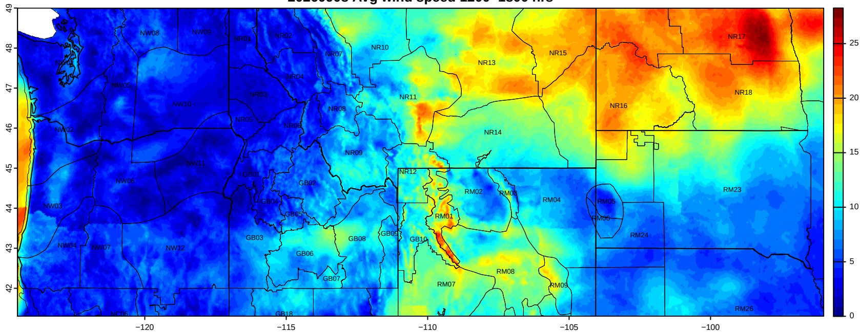
20260909 Avg wind speed 1200–1800 hrs
