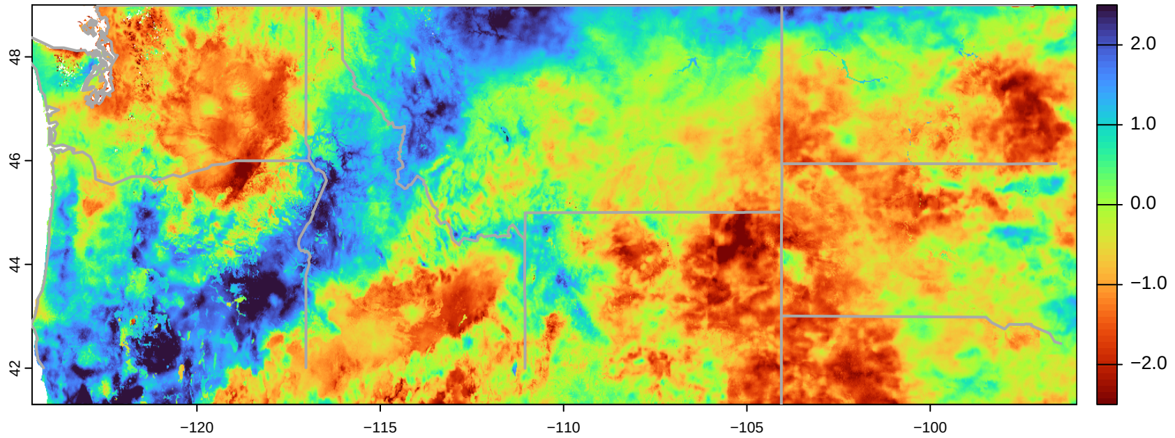
topofire soil moisture anomaly
