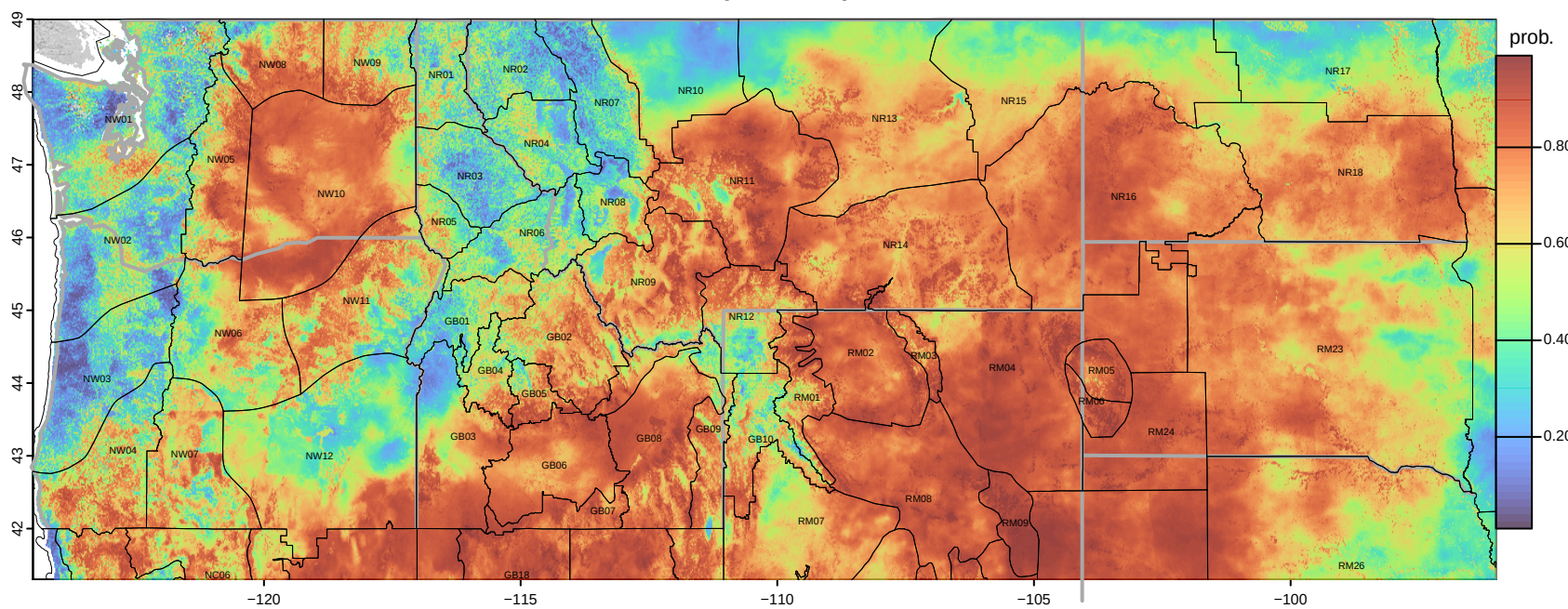
20260910 Probability. of fire spread > 70 acres
