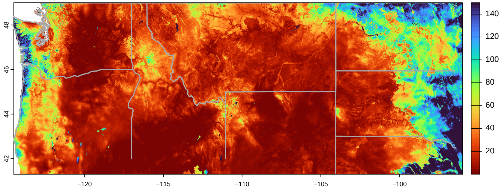
topofire raw soil moisture (mm)
