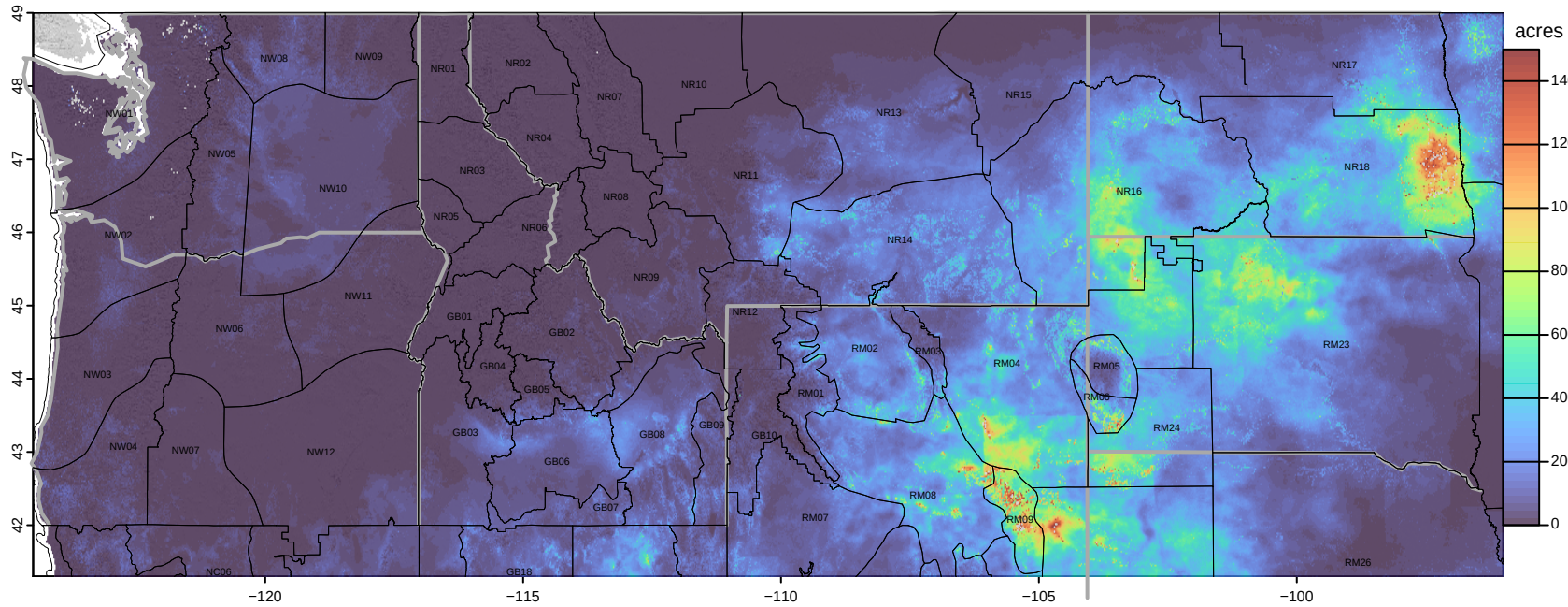
20260909 potential acres fire growth
