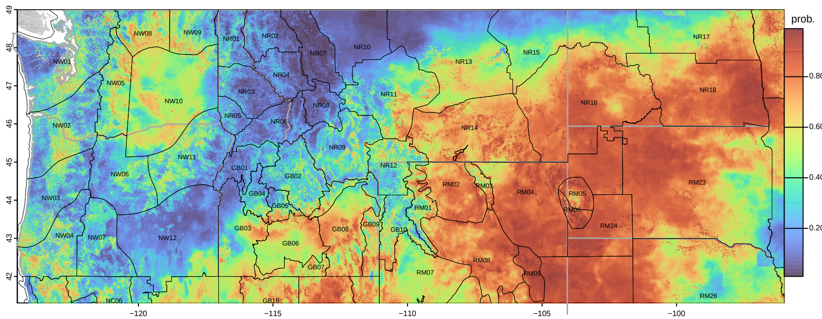
20260909 Probability. of fire spread > 70 acres
