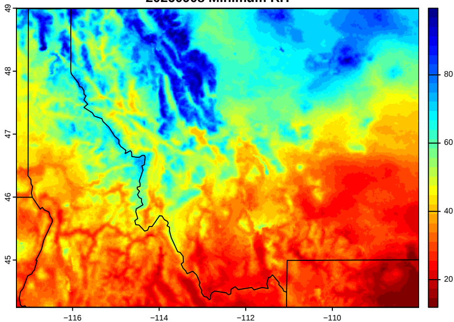
20260909 Minimum RH
