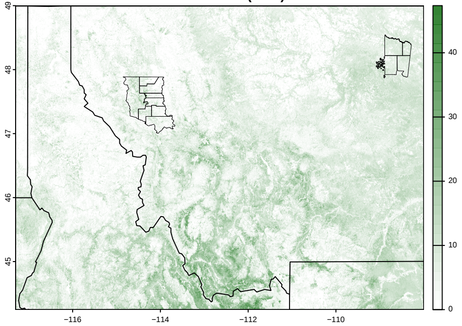
forest cover % (2023)
