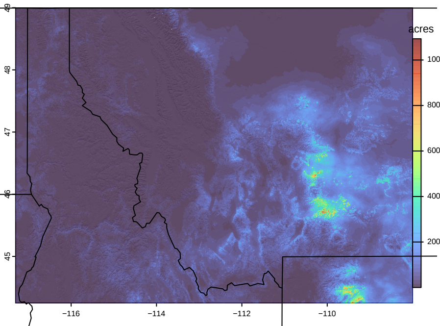
20260910 potential acres fire growth
