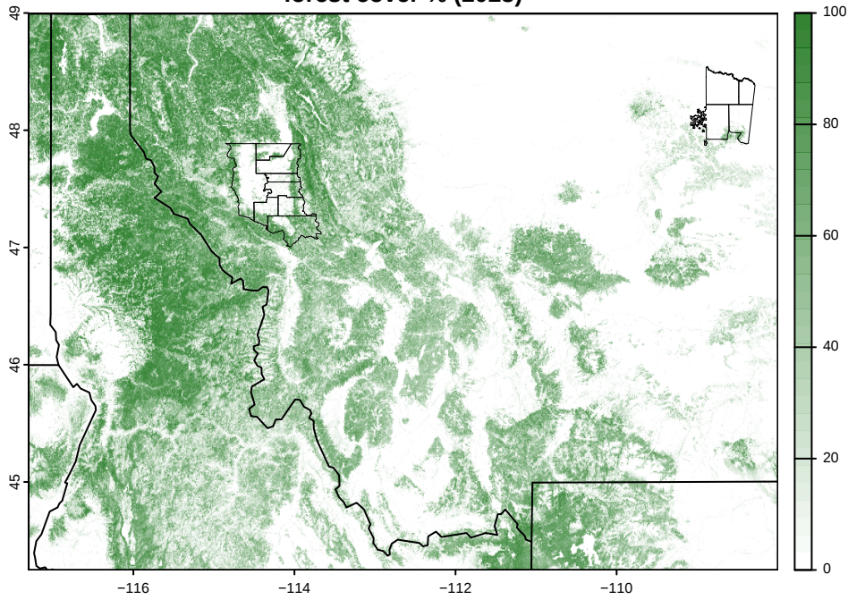
forest cover % (2023)
