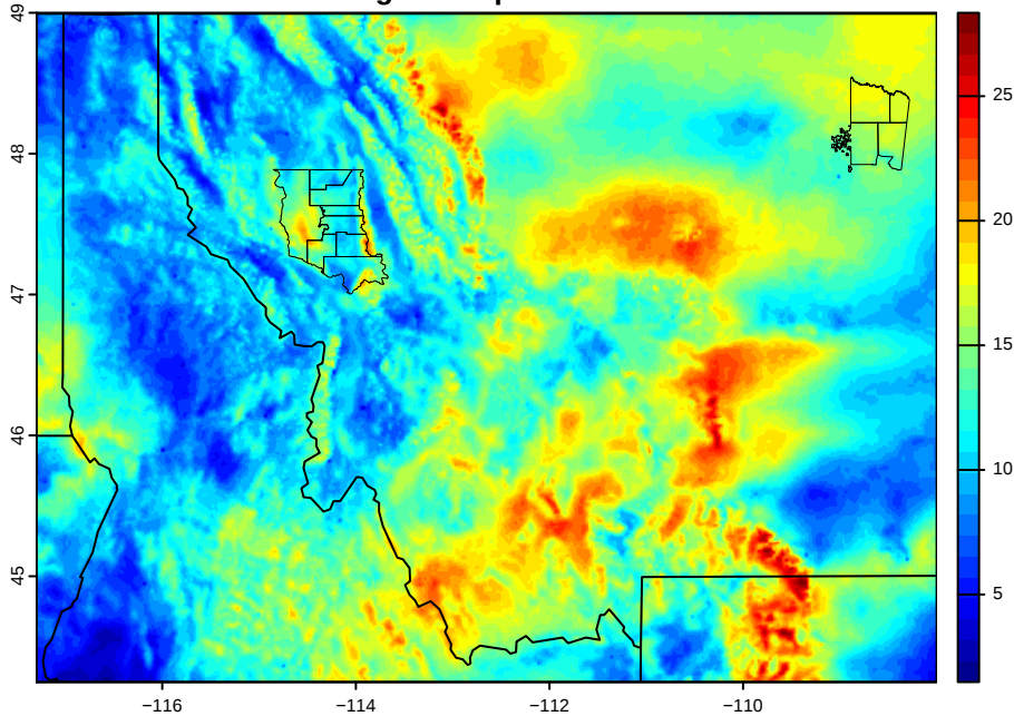
20260910 Avg wind speed 1200–1800 hrs
