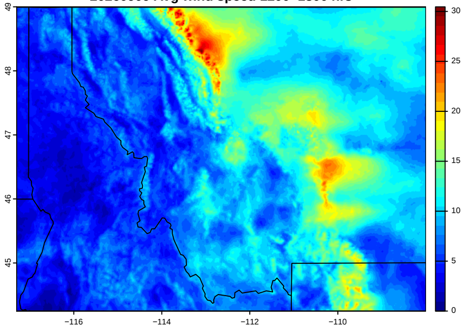
20260909 Avg wind speed 1200–1800 hrs
