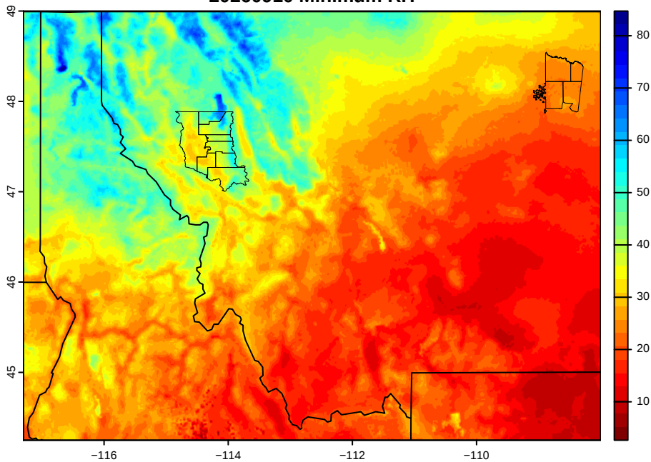
20260910 Minimum RH
