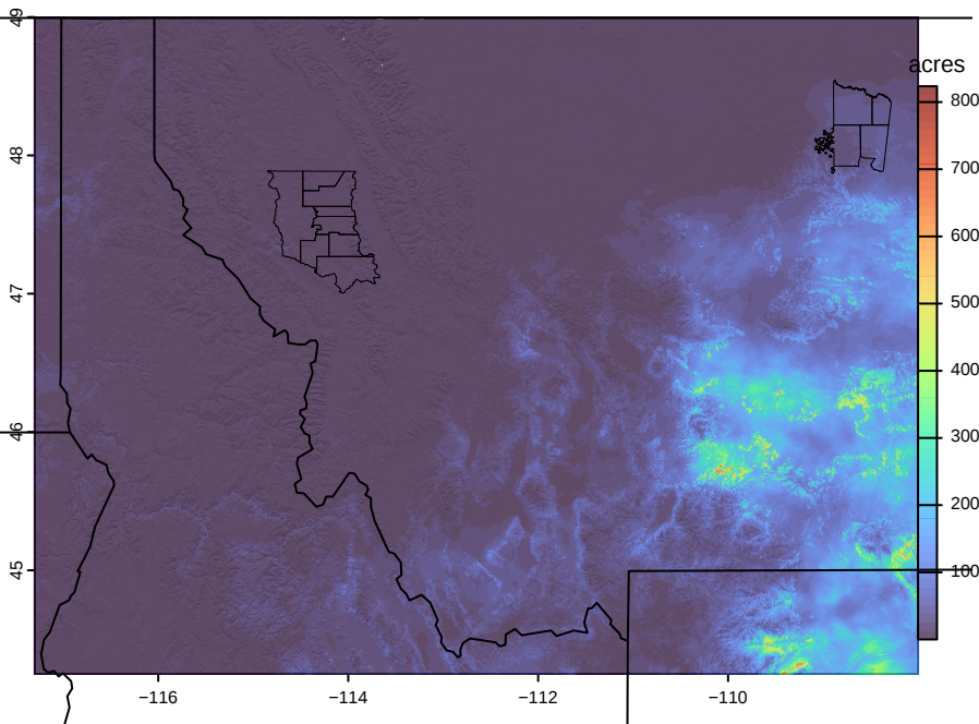
20260909 potential acres fire growth
