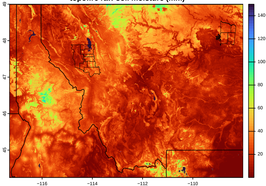
topofire raw soil moisture (mm)
