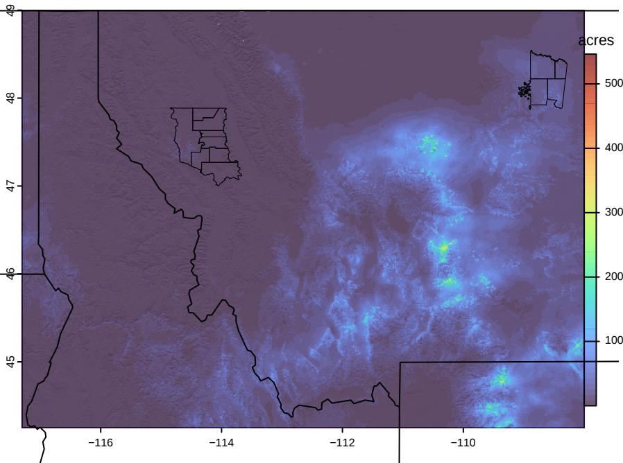
20260910 potential acres fire growth
