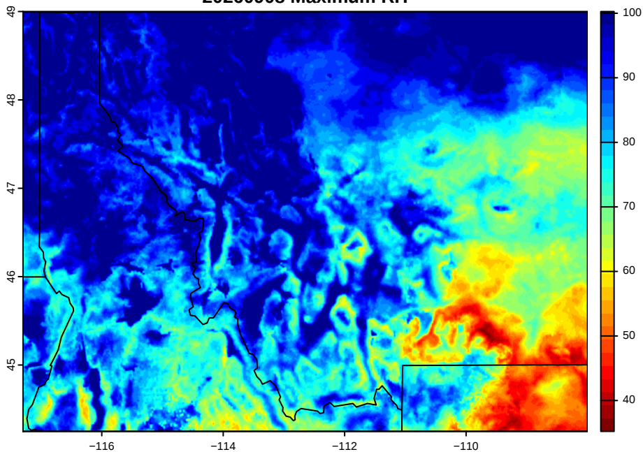
20260909 Maximum RH
