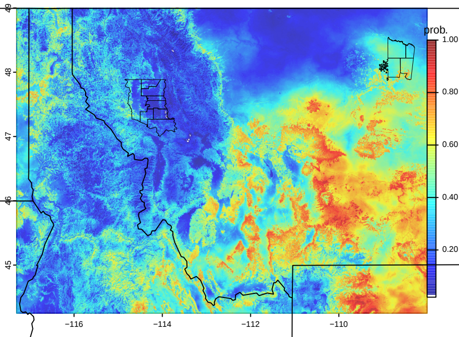
20260910 Probability. of fire spread > 70 acres
