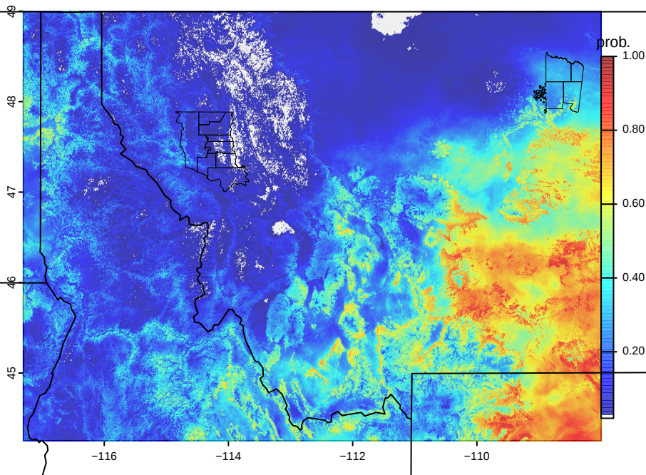
20260909 Probability. of fire spread > 70 acres
